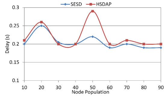
Fig. 4: Delay vs node population for the proposed SEDS with HSDAP
