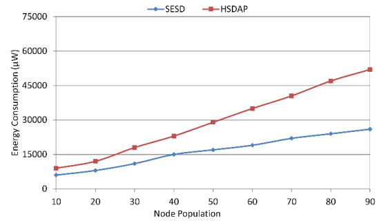
Fig. 5: Energy Consumption Analysis for the proposed SEDS with HSDAP
