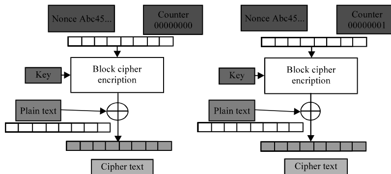
Fig. 2: Counter mode encryption
