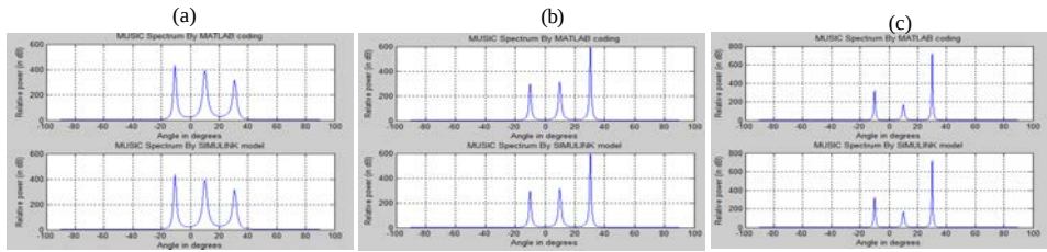
Fig. 10: MUSIC angular spectrum for different values of Number of Elements: a) N = 5 ; b) N = 6 ; c) N = 7
