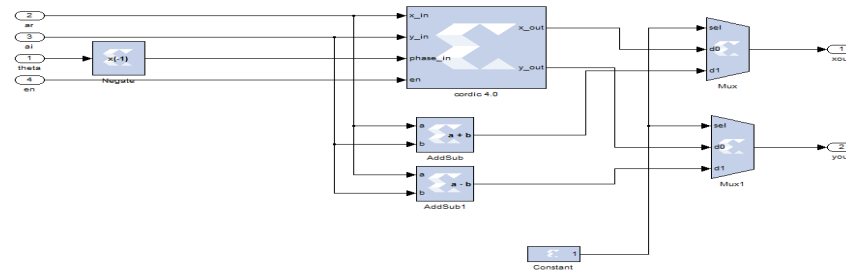
Fig. 3: TSA with XSG blocks
