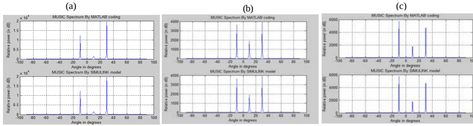
Fig. 8: MUSIC angular spectrum for different values of number of elements: a) N = 5 ; b) N = 6 ; c) N = 7
