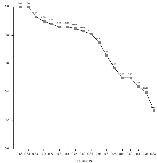
Fig. 10: Precision-Recall graph
