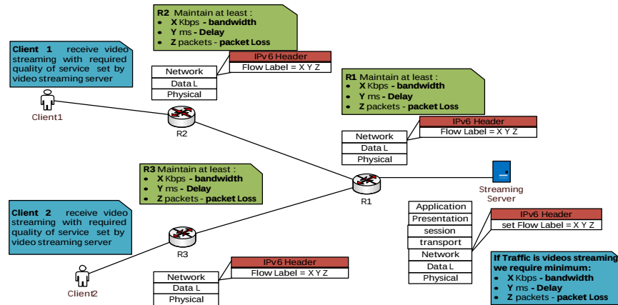
Fig. 3: 20 bit flow label field optimization
