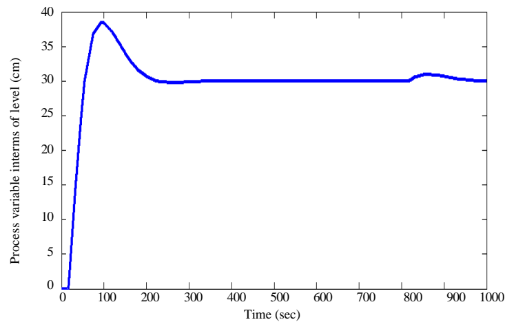
Fig. 17: Process variable versus time graph for the regulatory operation of the genetic algorithm tuned PI controller for the conical tank process with the height 30 cm with +10% load changes after 800 sec
