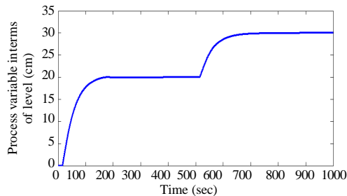
Fig. 11: Process variable versus time graph for the servo operation of the neuro tuned PI controller for the conical tank process with the height of 20 cm and further the height is increased 10 cm
