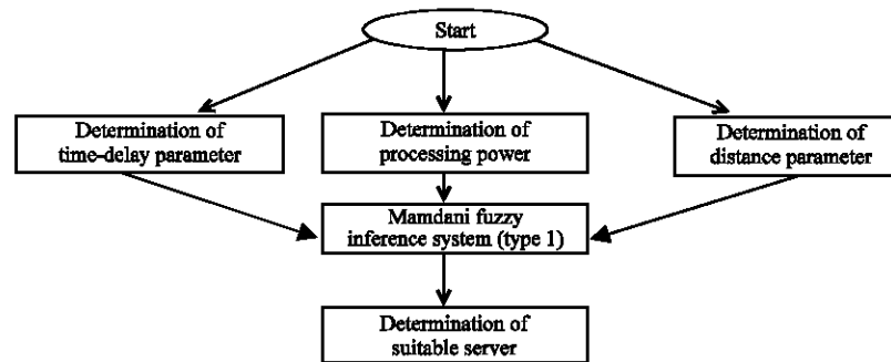
Fig. 1: Suggested algorithm
