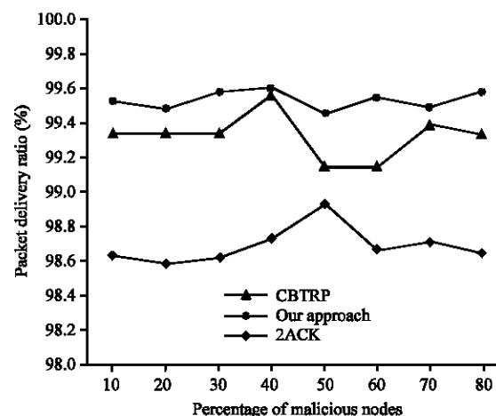
Fig. 2: Packet delivery ratio of our approach, CBTRP and 2ACK
