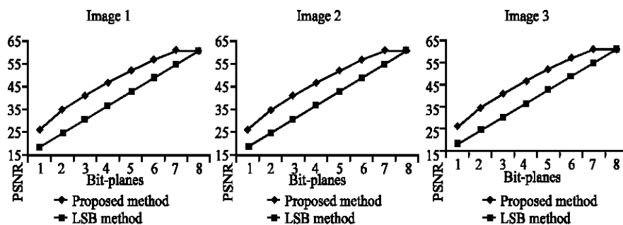
Fig. 10: PSNR value of the proposed method and LSB method for different bit-planes
