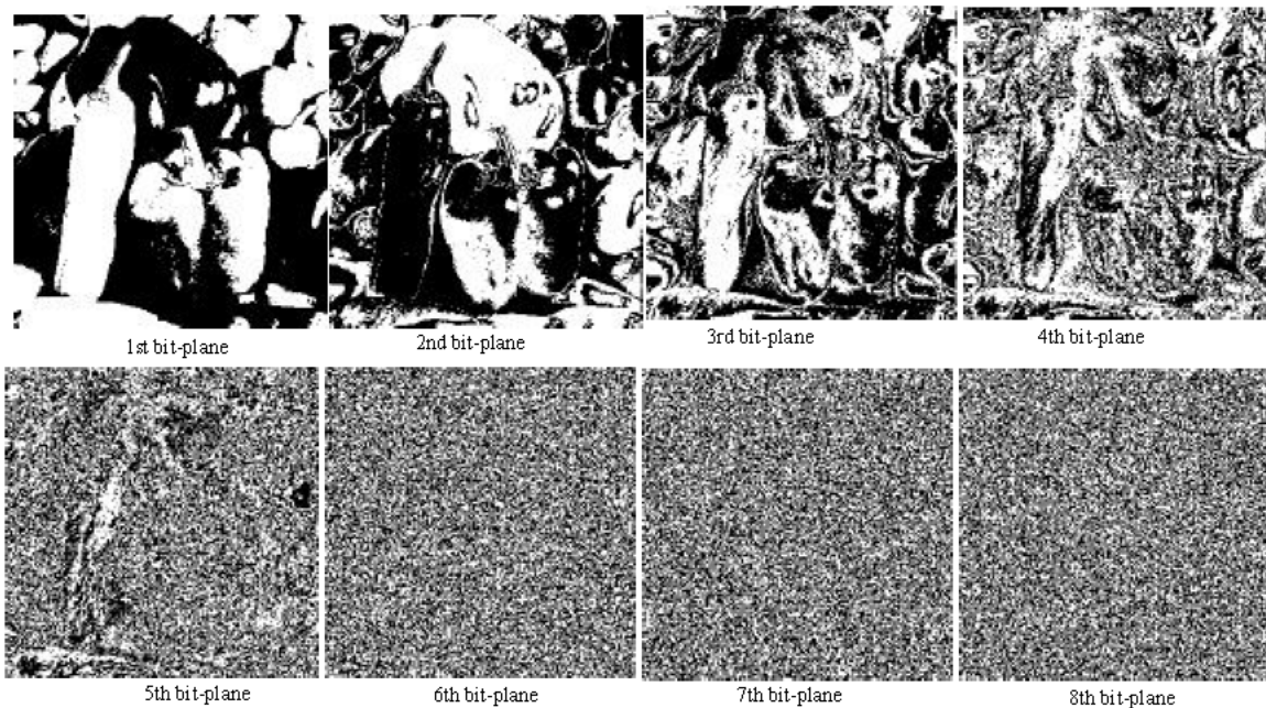
Fig. 2: Eight bit-planes from most significant to least significant bits
