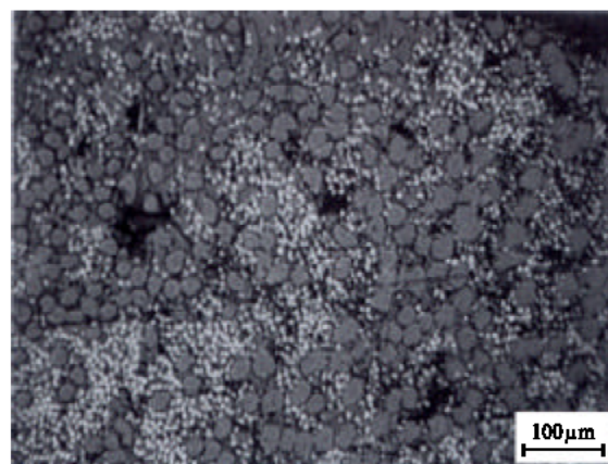
Fig. 1: Micrography of one intermingled with powder and Polyamide carbon fibers (Bernet et al. , 1999)
