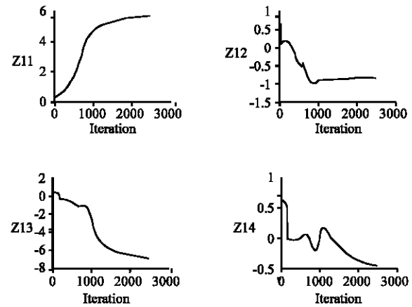
Fig. 13: The variation of the four first values of the connection weights between the hidden layer and the output layer
