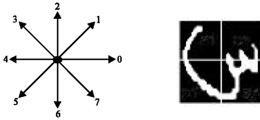
Fig. 11: Principle of the coding of freeman
