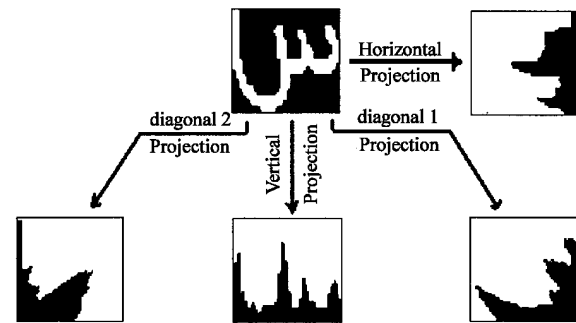
Fig. 6: The four projections of the character SIN
