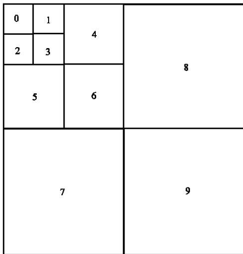
Fig. 6: 8×8 DCT block taken as three-scale tree with ten-subband decomposition
