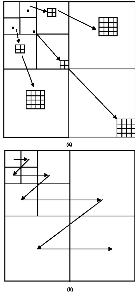
Fig. 4: (a) Structure of zerotrees and (b) Scanning order of subbands for encoding
