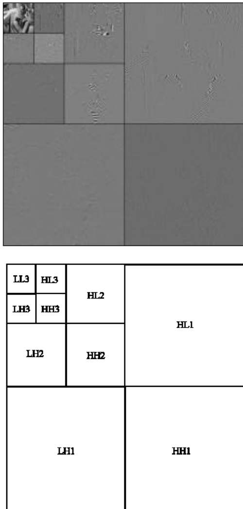
Fig. 3: Decomposition results from the third stage
