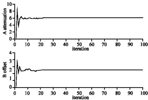
Fig. 6: Estimation the values of attenuation and offset
