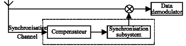
Fig. 4: The synchronization schema with compensator before the receiver
