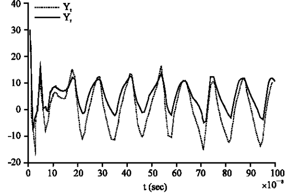
Fig. 3: Synchronization between transmitter and receiver in satellite channel with attenuation A = 2 and offset B = 6
