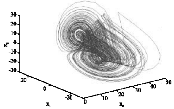
Fig. 1: The typical Chen Chaotic attractors
