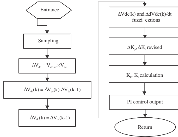
Fig. 6: Flow chart of parameters online regulation
