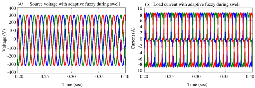
Fig. 12(a, b): Simulation result for V_{\text{source}} and I_{\text{load}}
