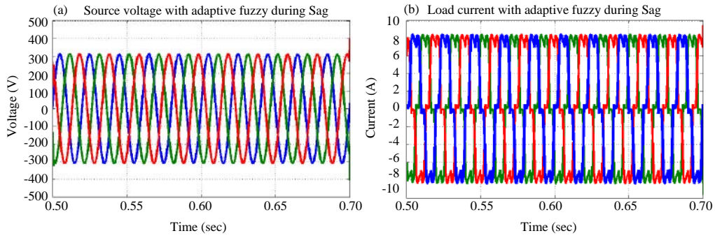
Fig. 11(a, b): Simulation result for V_{\text{source}} and I_{\text{load}}
