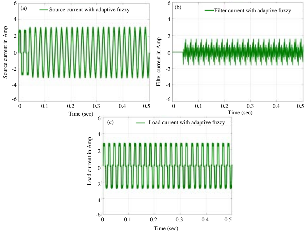
Fig. 10(a-c): Simulation result for I_{\text{source}} , I_{\text{filter}} and I_{\text{load}}
