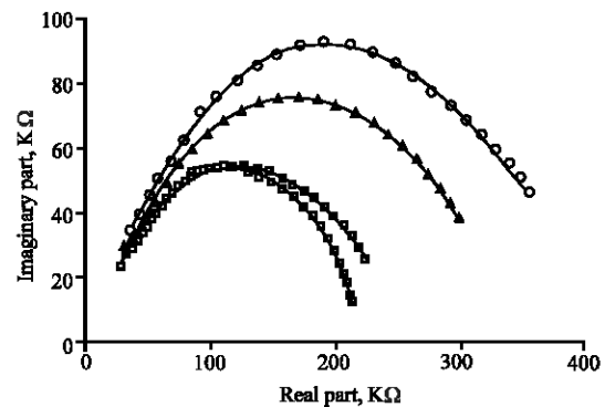
Fig. 3: Typical impedance spectra of the first leaf during growth. Symbols: \blacklozenge =/April 25, \blacktriangledown =/May 3, \blacksquare =/May 9 and \bullet =/May 15. Frequency increases from right (0.5 kHz) to left (500 kHz)
