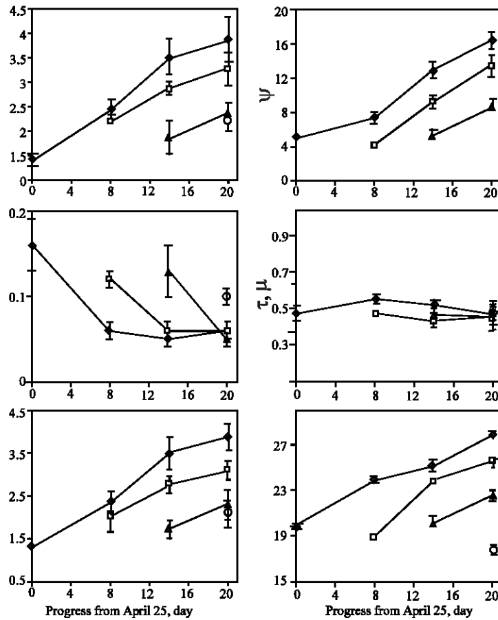
Fig. 4: Changes in the parameters for a single-DCE model of the tea leaf by impedance analysis and dry matter content in the leaf. Symbols: \blacklozenge = 1st leaf, \square = 2nd leaf, \blacktriangle = 3rd leaf and \circ = 4th leaf. The parameters r_\infty , r_i and r_1 are resistances, \tau is the distribution coefficient of the relaxation time ( \tau ). The progress from April 25 is shown on the x-axis. Each point is the mean of 5 measurements and the bars indicate standard deviation
